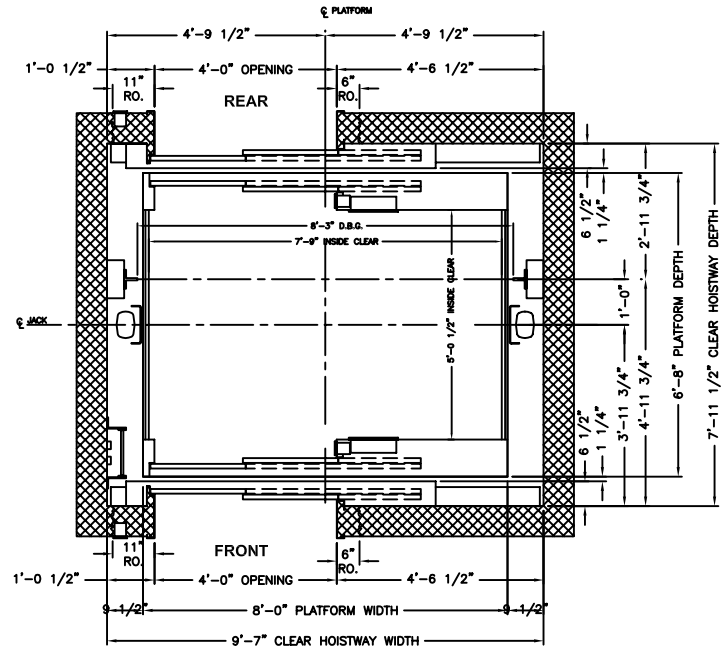
PLAN VIEW HOISTWAY
