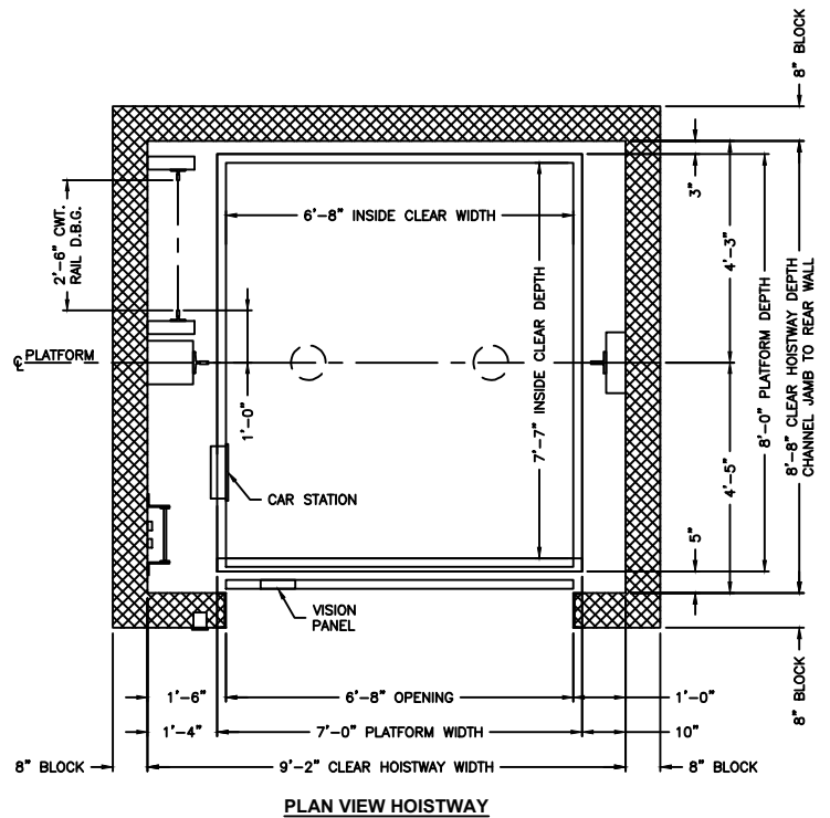
PLAN VIEW HOISTWAY
