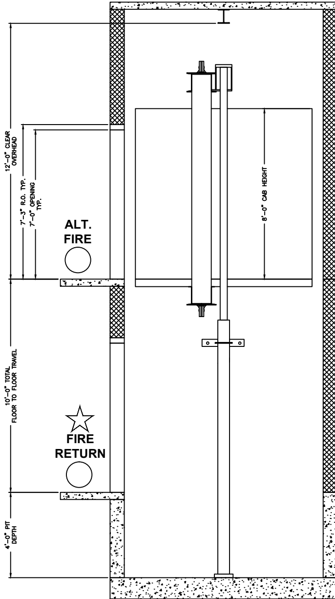
ELEVATION VIEW HOISTWAY
