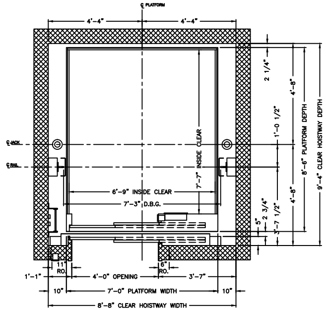
PLAN VIEW HOISTWAY
