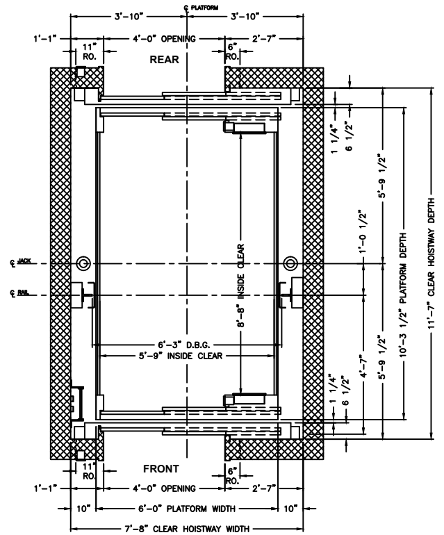
PLAN VIEW HOISTWAY
