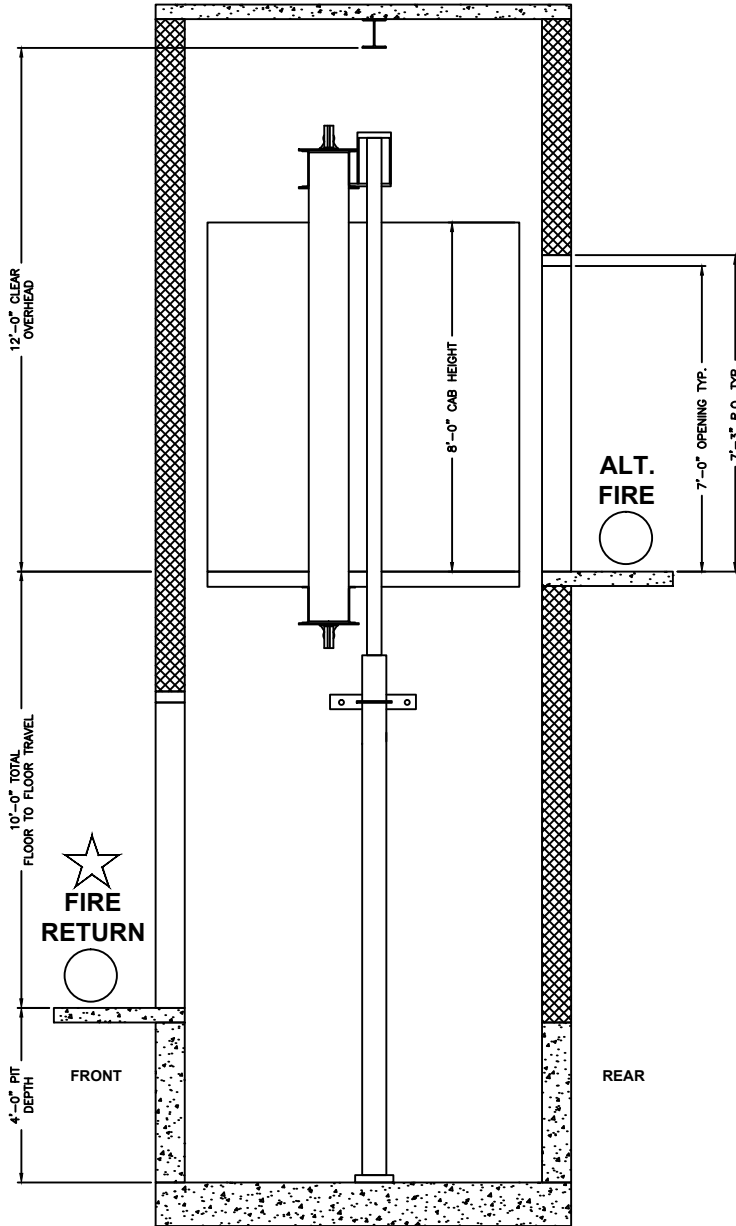
ELEVATION VIEW HOISTWAY
