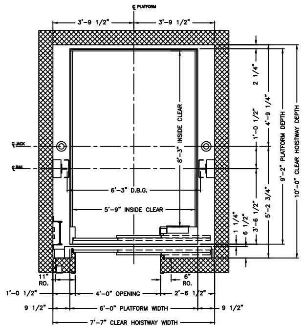
PLAN VIEW HOISTWAY
