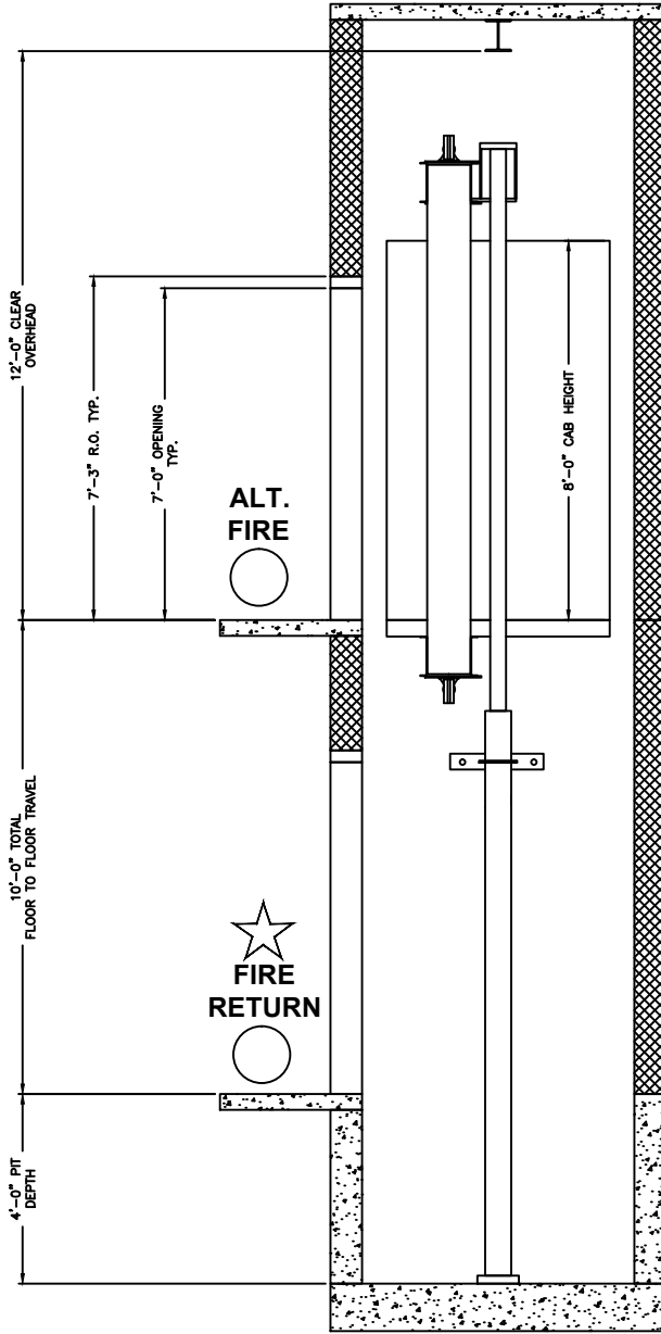
ELEVATION VIEW HOISTWAY
