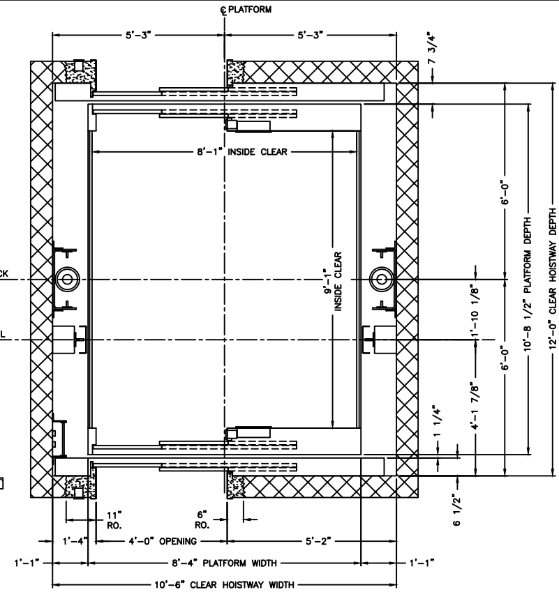
PLAN VIEW HOISTWAY
