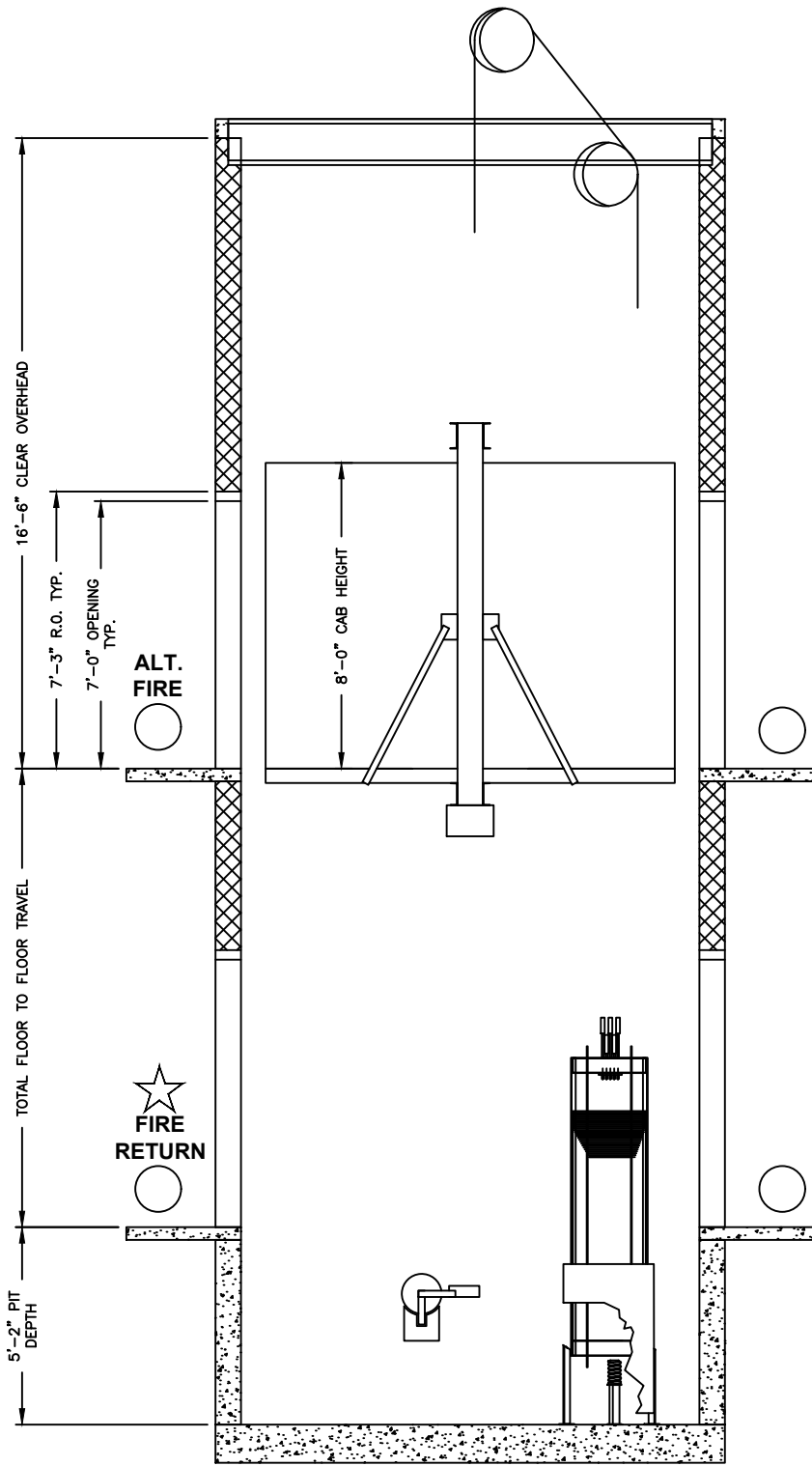
HOISTWAY SECTION
