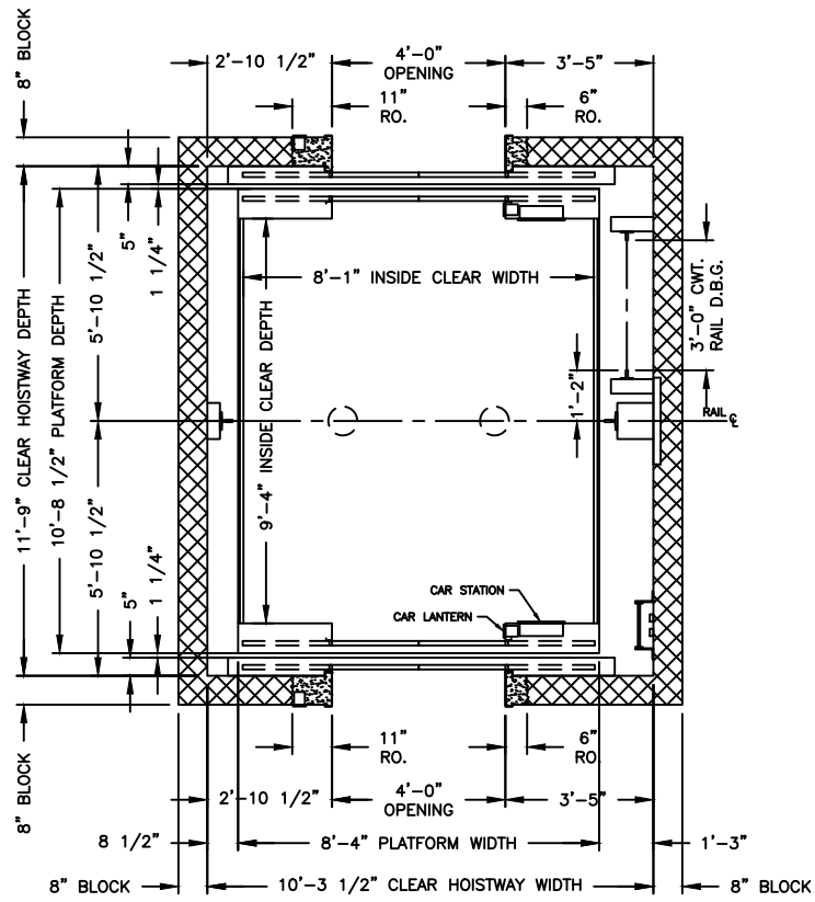
HOISTWAY PLAN
