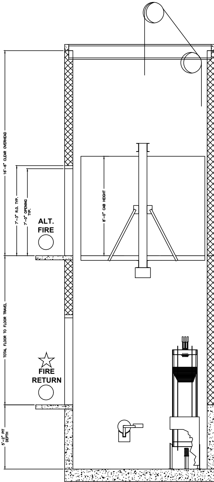
HOISTWAY SECTION
