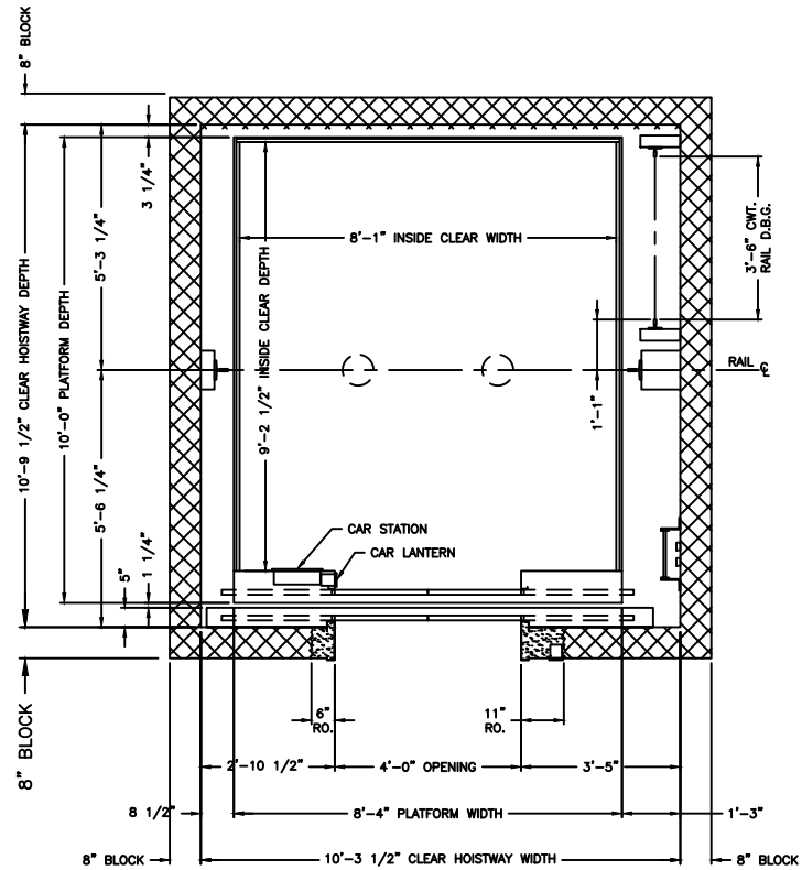
HOISTWAY PLAN
