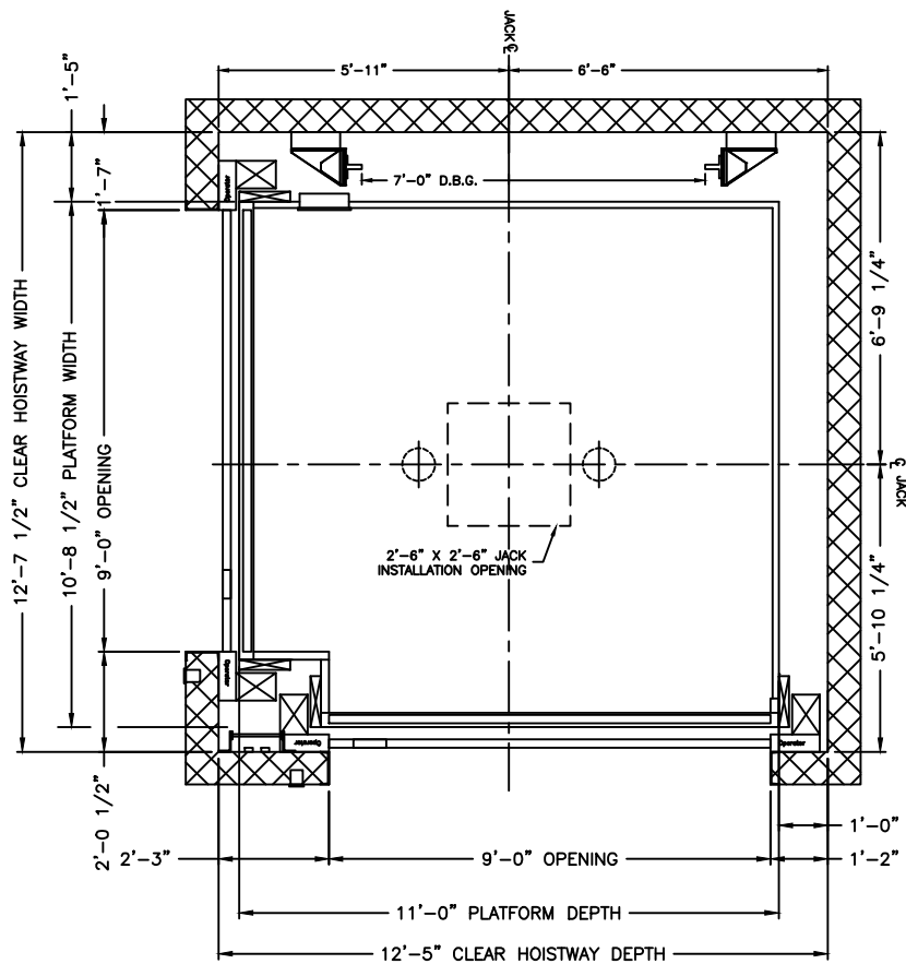
PLAN VIEW HOISTWAY
