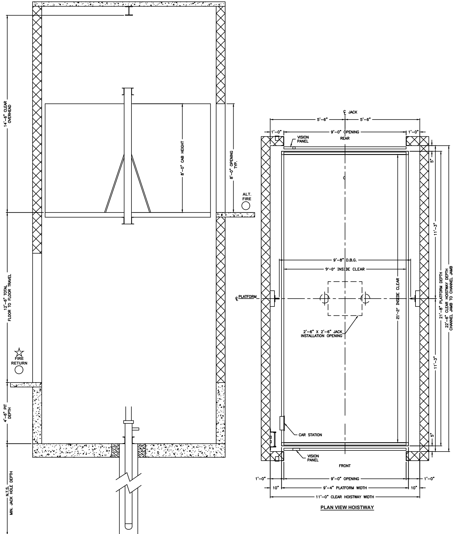
8000# CAPACITY F/R
