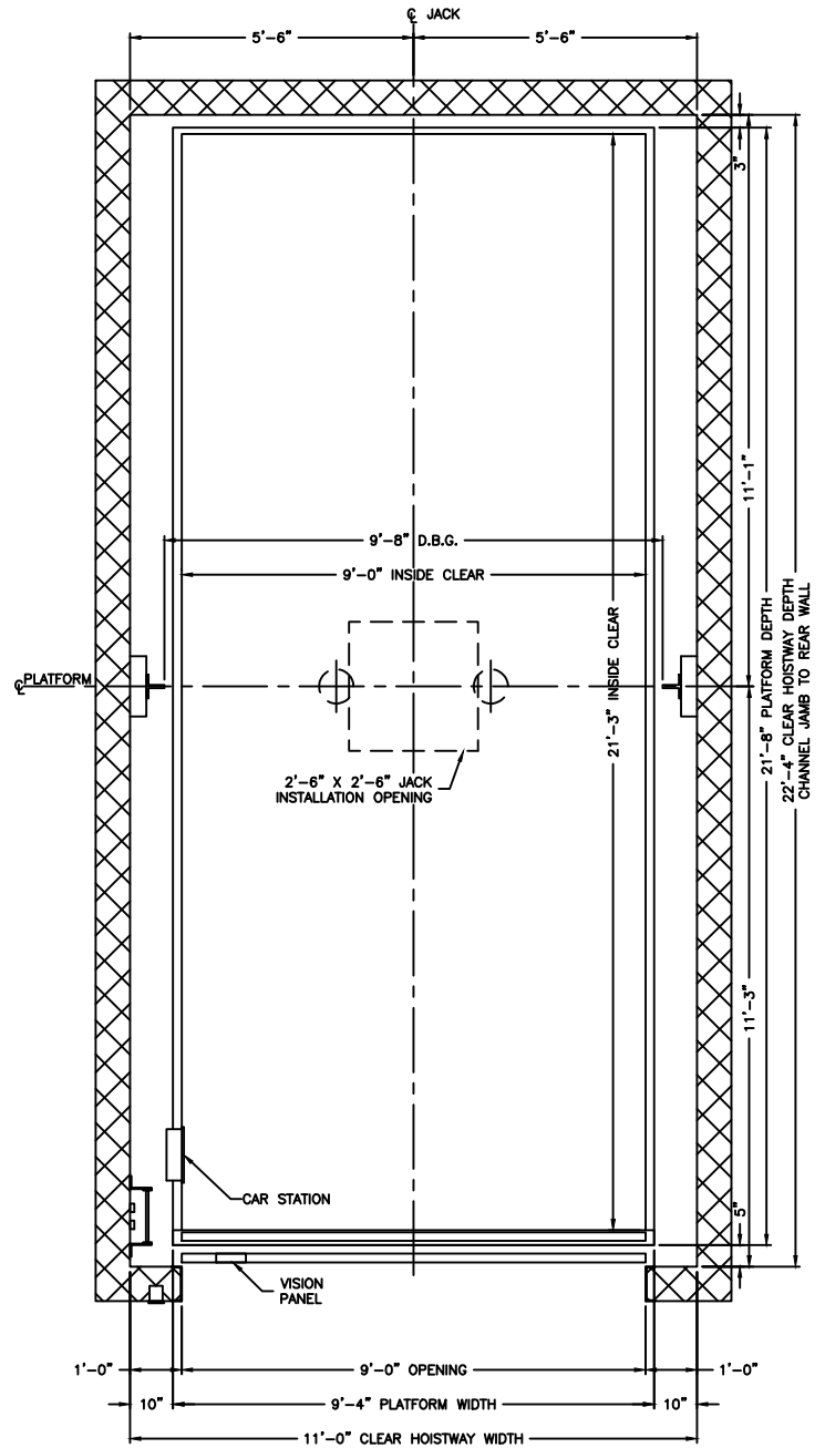
PLAN VIEW HOISTWAY
