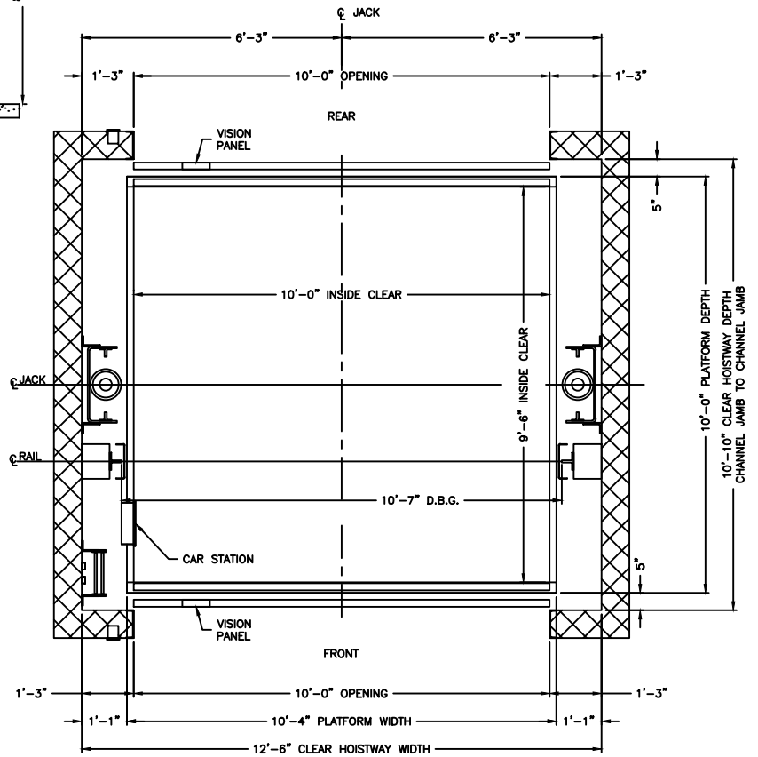
PLAN VIEW HOISTWAY
