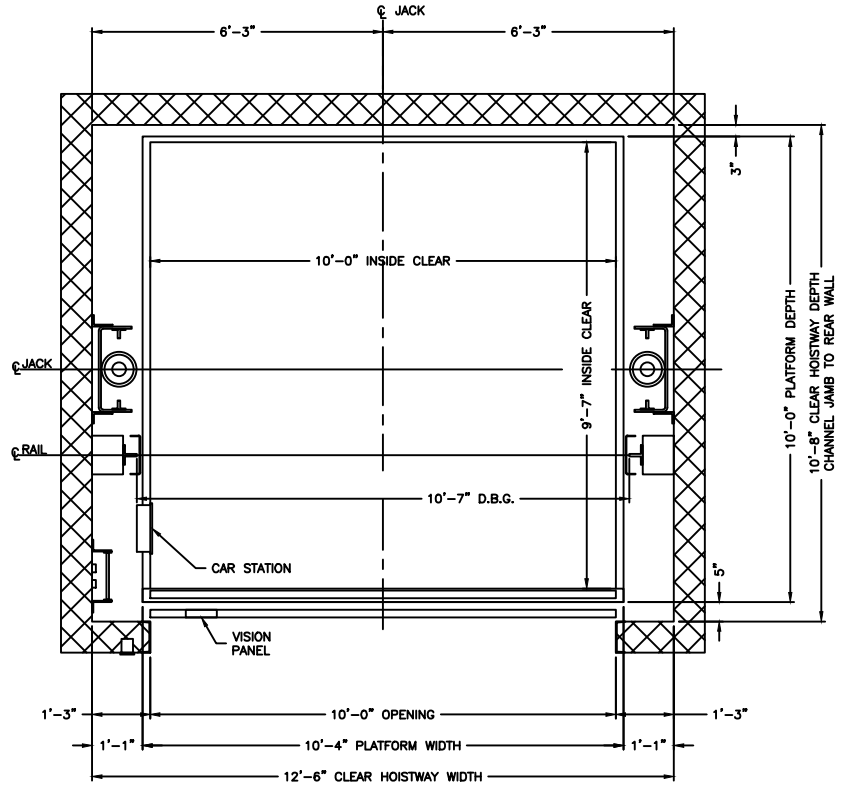
PLAN VIEW HOISTWAY
