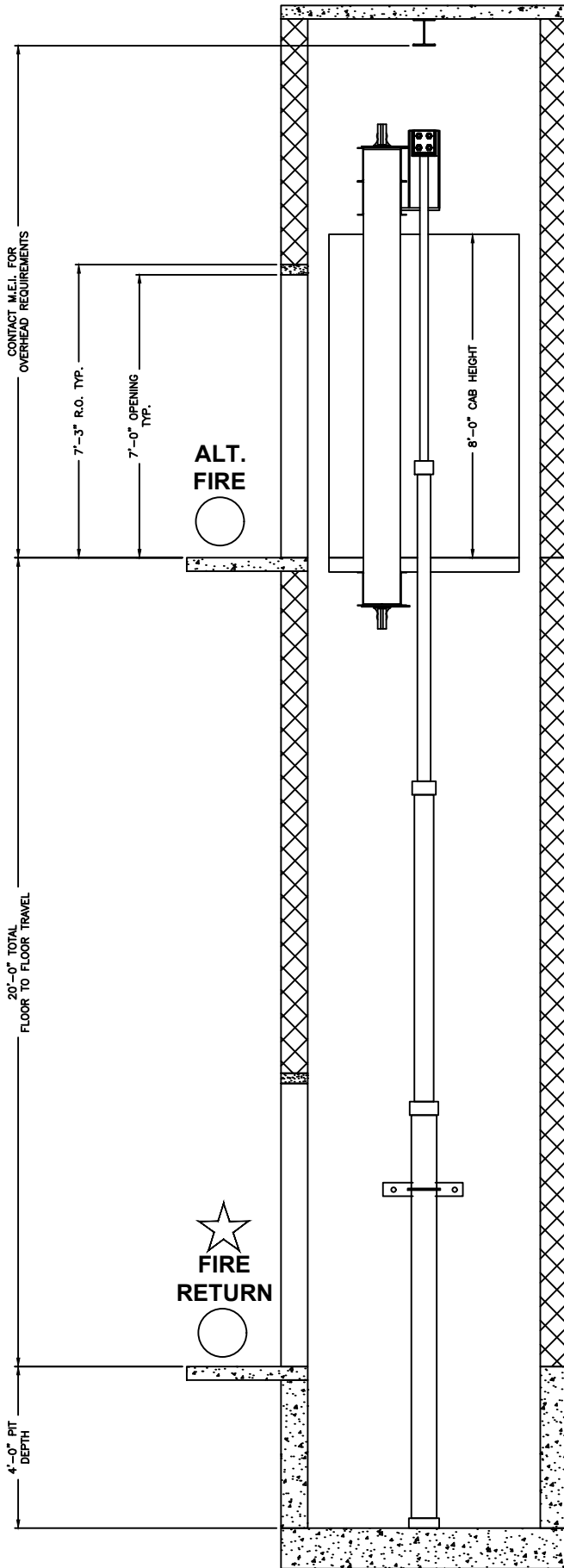
ELEVATION VIEW HOISTWAY
