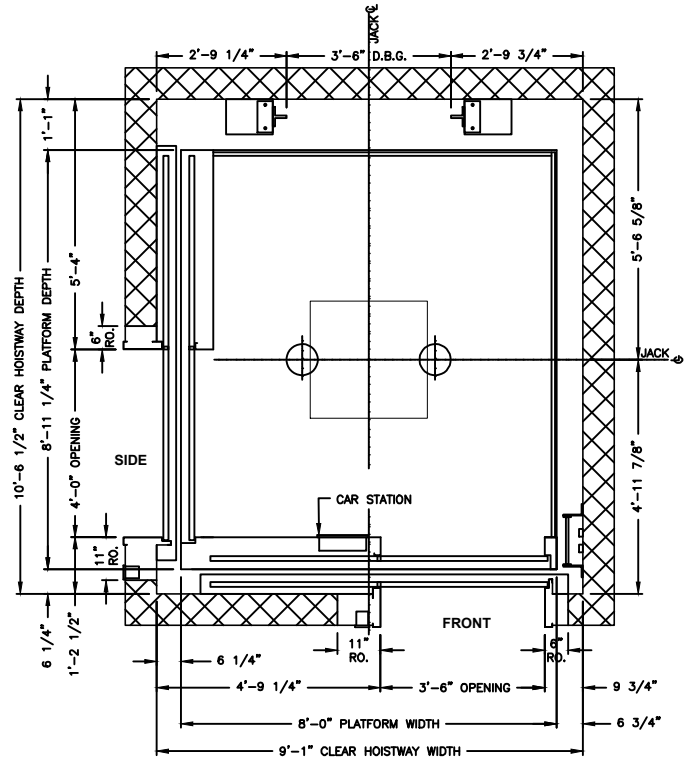
PLAN VIEW HOISTWAY
