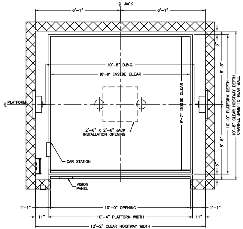
PLAN VIEW HOISTWAY
