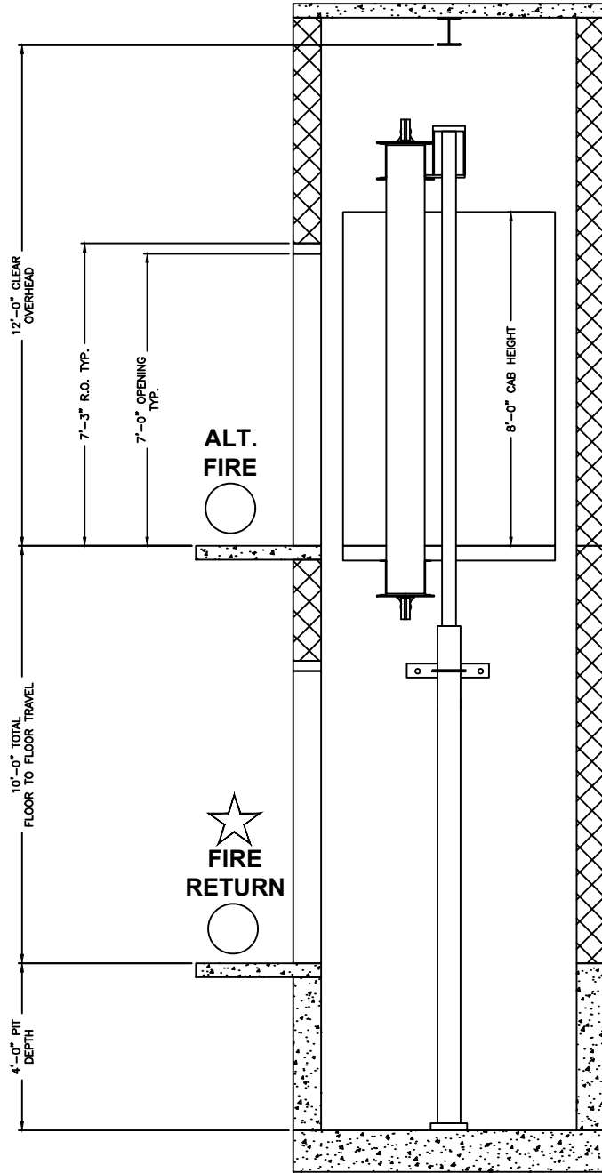
ELEVATION VIEW HOISTWAY
