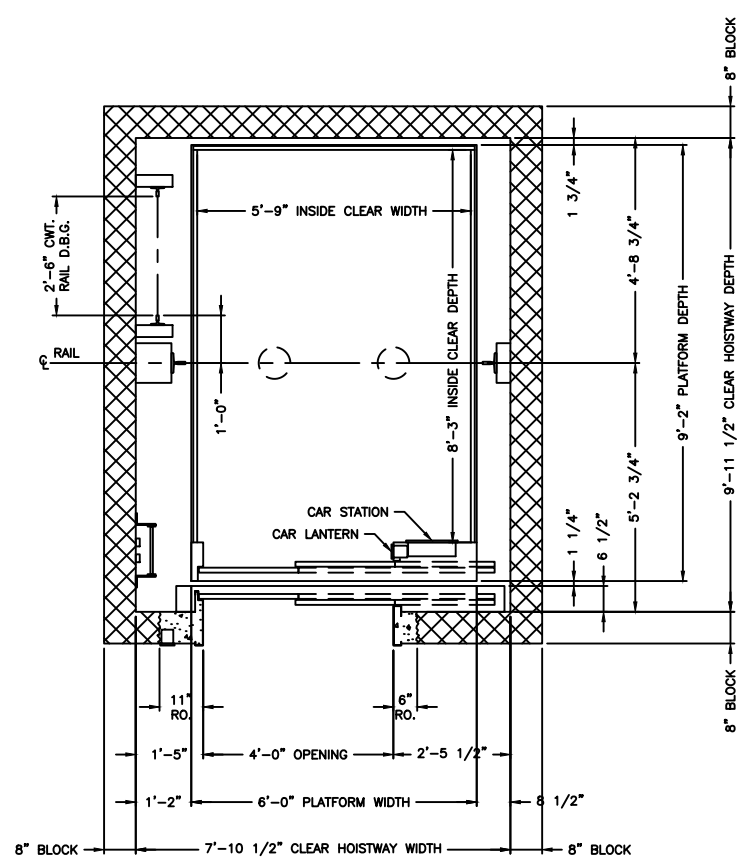
PLAN VIEW HOISTWAY
