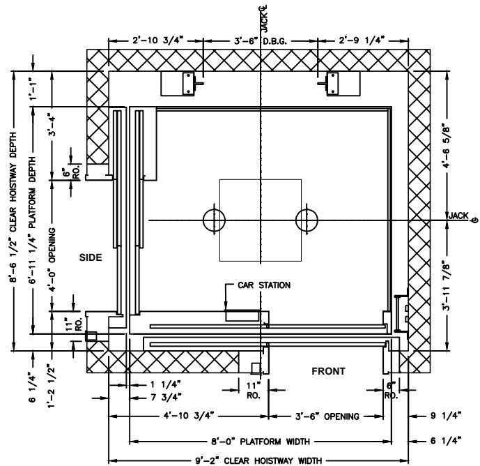
PLAN VIEW HOISTWAY
