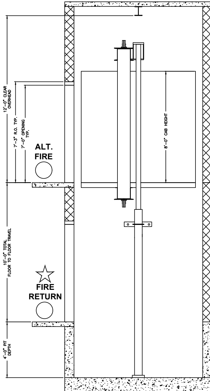
ELEVATION VIEW HOISTWAY
