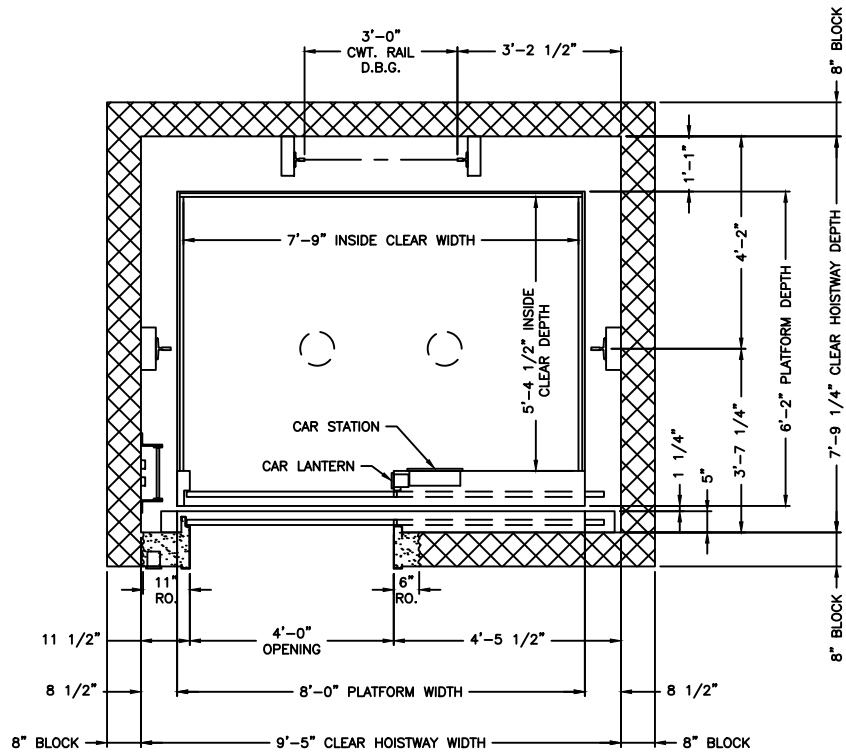
PLAN VIEW HOISTWAY
