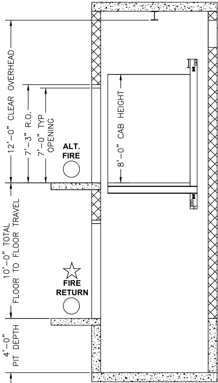
SECTION A-A ELEVATION VIEW
