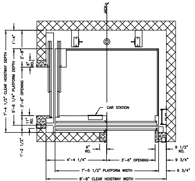
PLAN VIEW HOISTWAY
