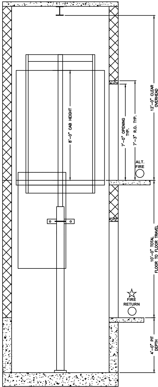
ELEVATION VIEW HOISTWAY
