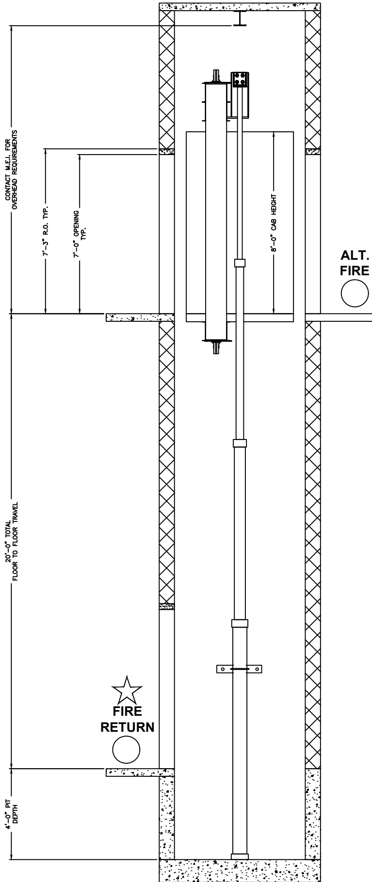
ELEVATION VIEW HOISTWAY
