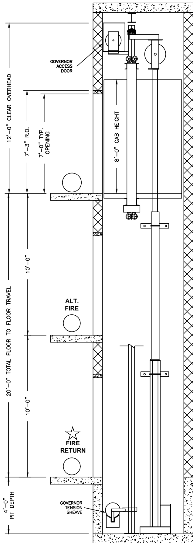
SECTION A-A ELEVATION VIEW
