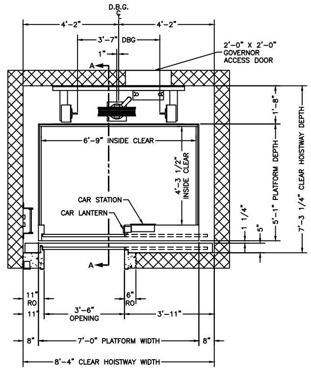
PLAN VIEW HOISTWAY
