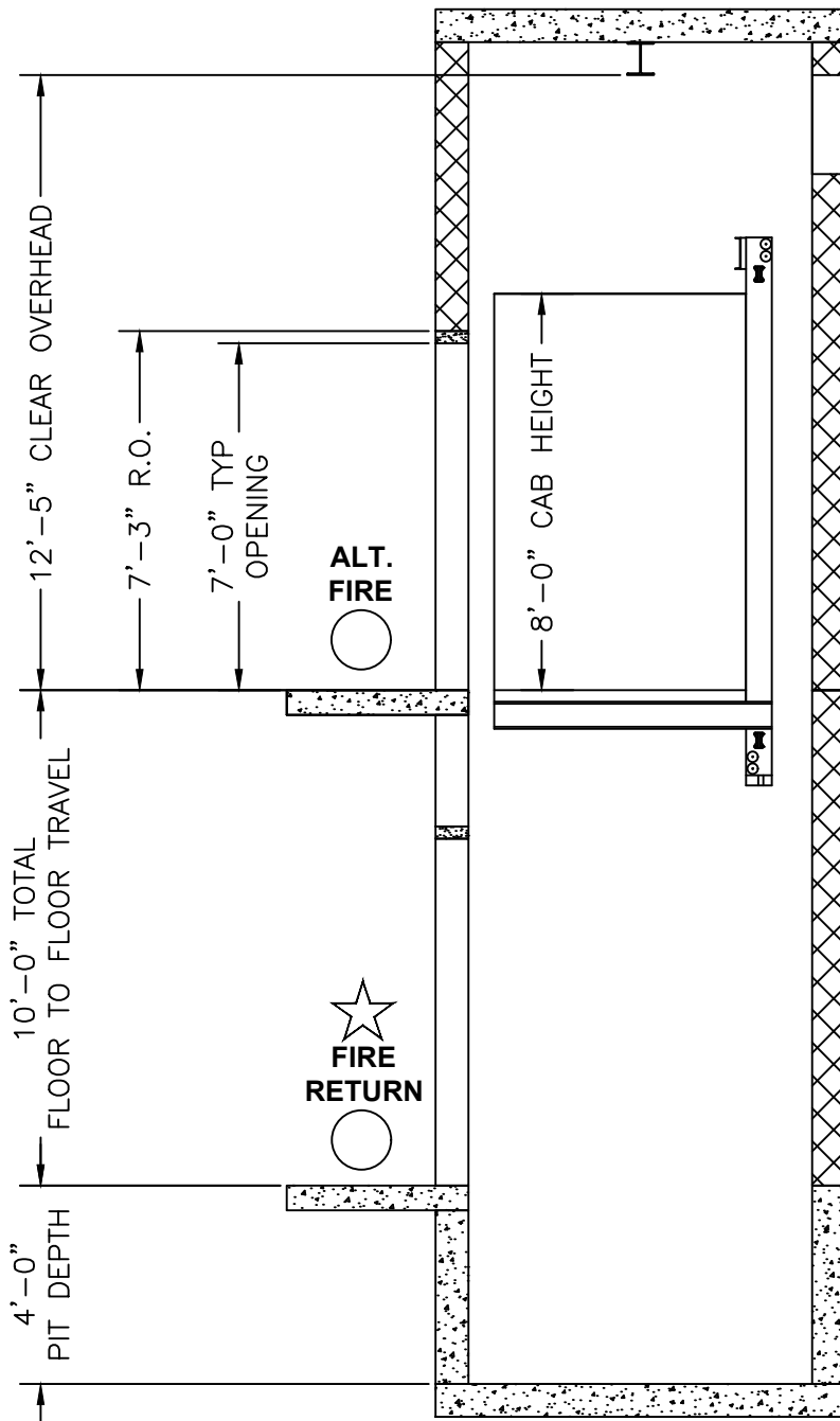
SECTION A-A ELEVATION VIEW
