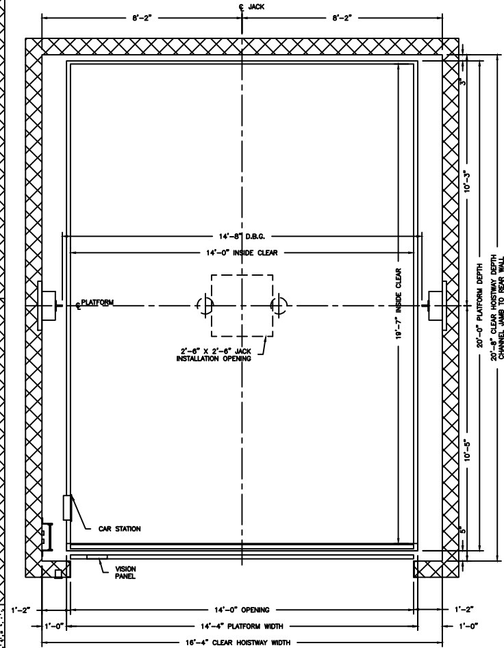
PLAN VIEW HOISTWAY
