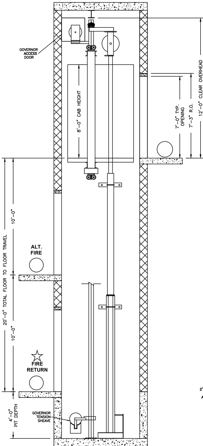
SECTION A-A ELEVATION VIEW
