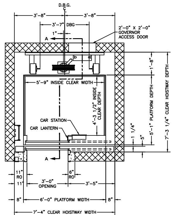
PLAN VIEW HOISTWAY
