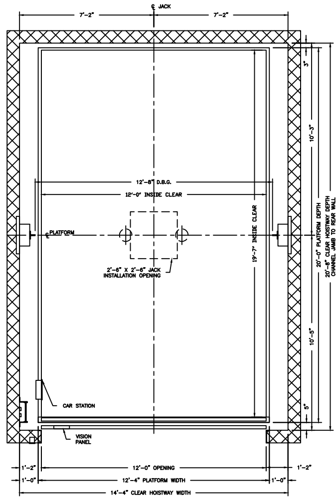
PLAN VIEW HOISTWAY
