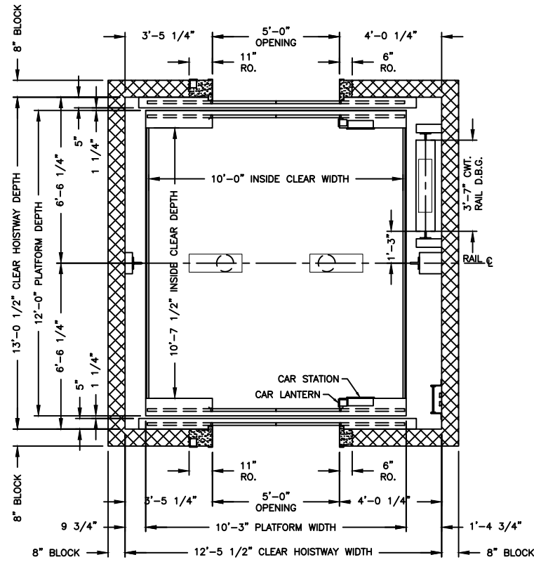
HOISTWAY PLAN
