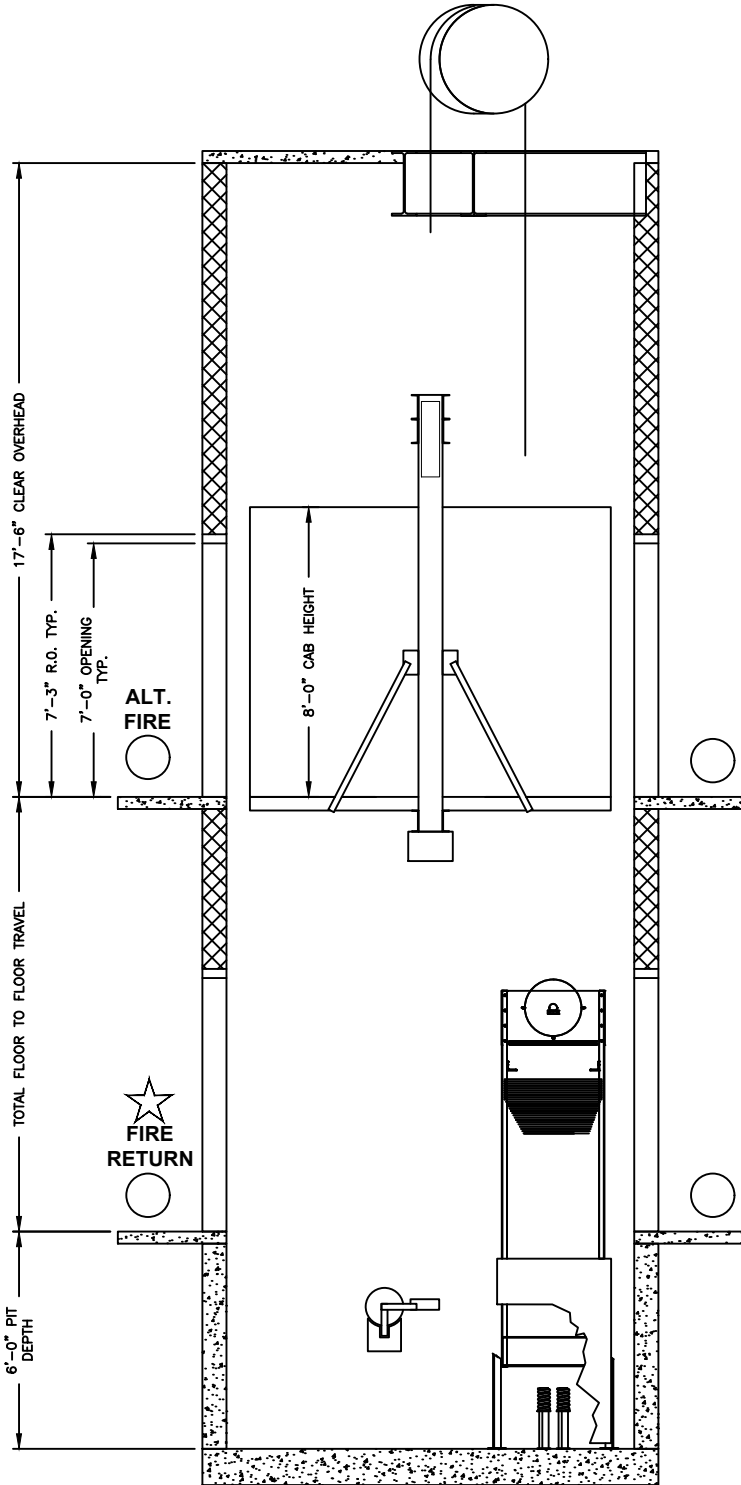
HOISTWAY SECTION
