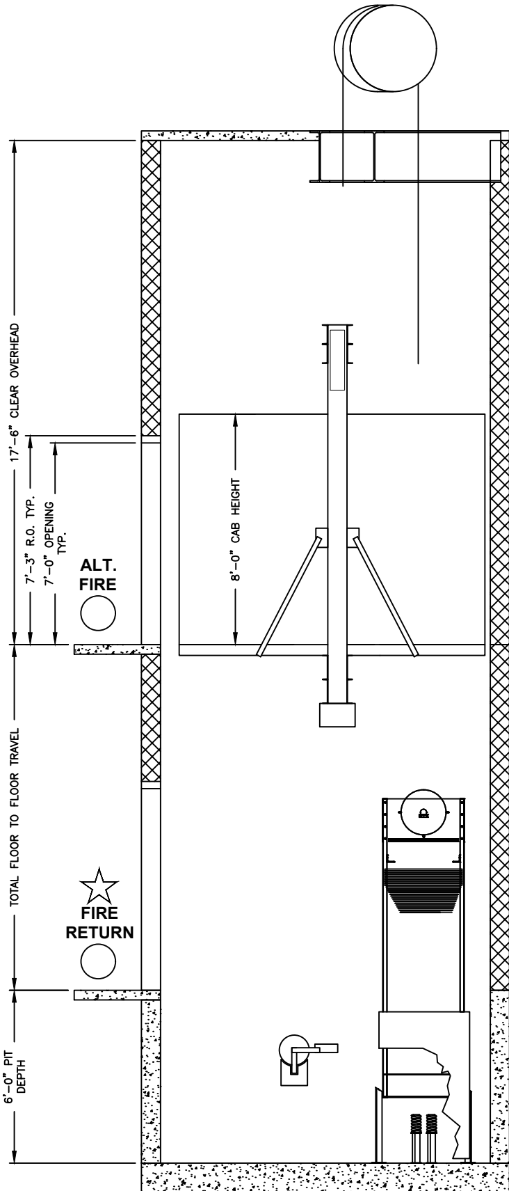
HOISTWAY SECTION
