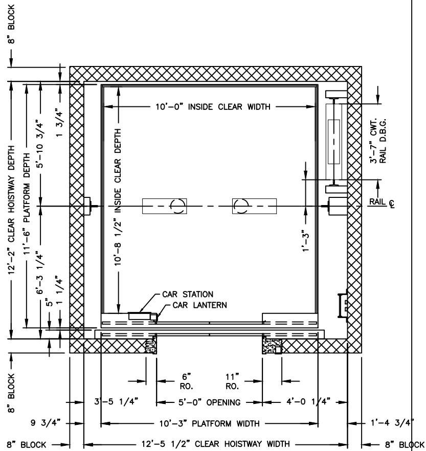
HOISTWAY PLAN
