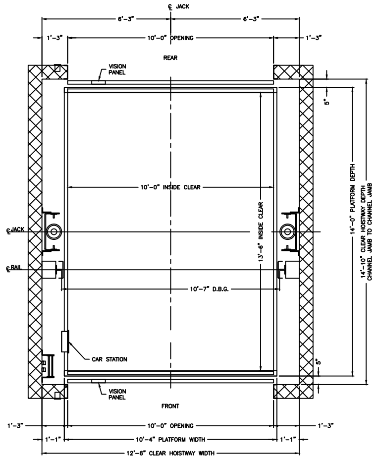
PLAN VIEW HOISTWAY
