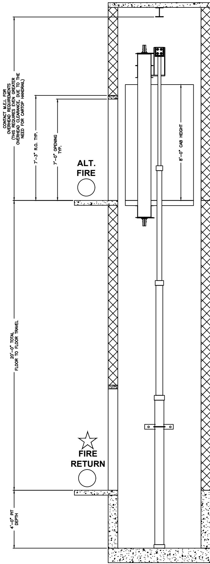
ELEVATION VIEW HOISTWAY
