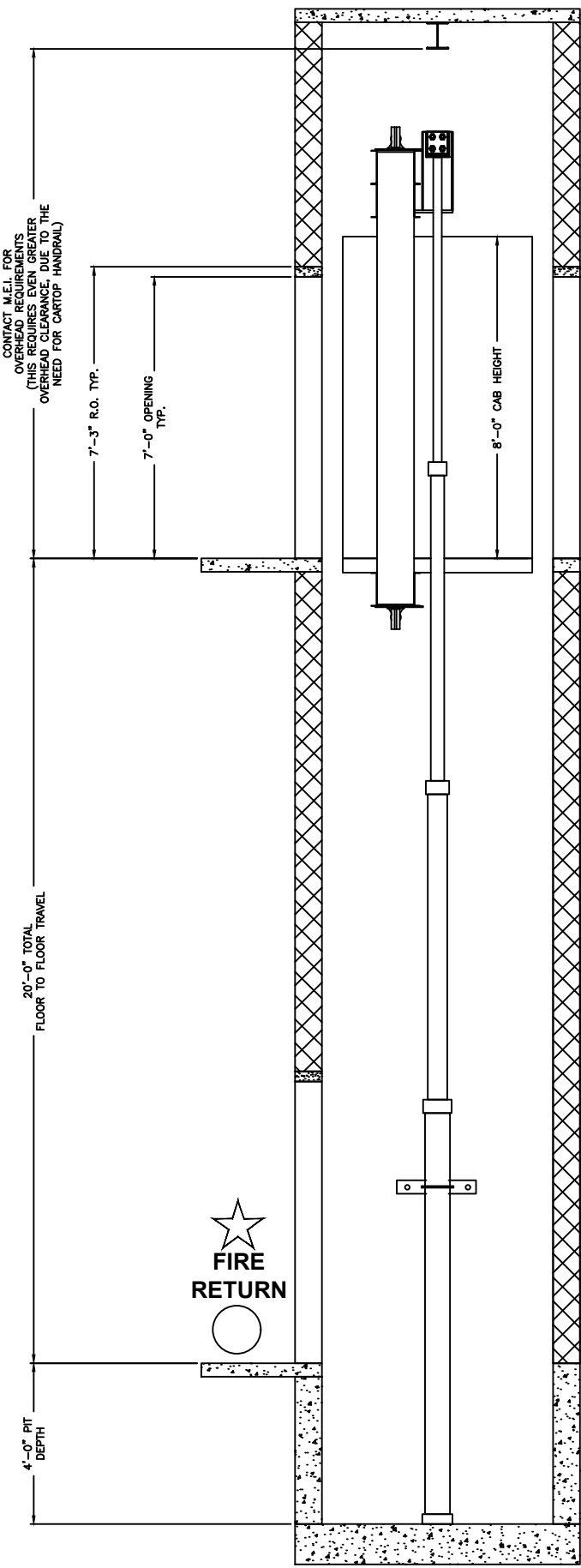
ELEVATION VIEW HOISTWAY
