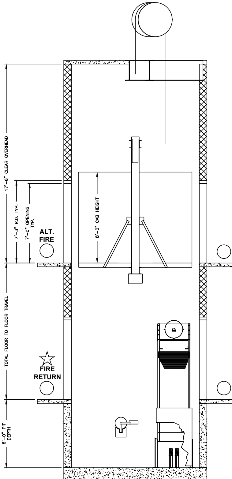
HOISTWAY SECTION
