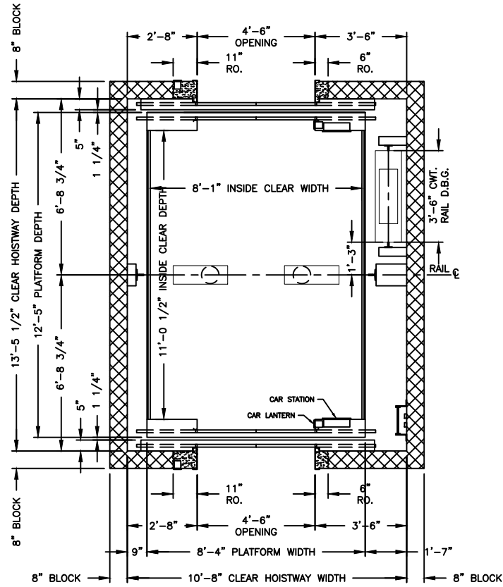
HOISTWAY PLAN
