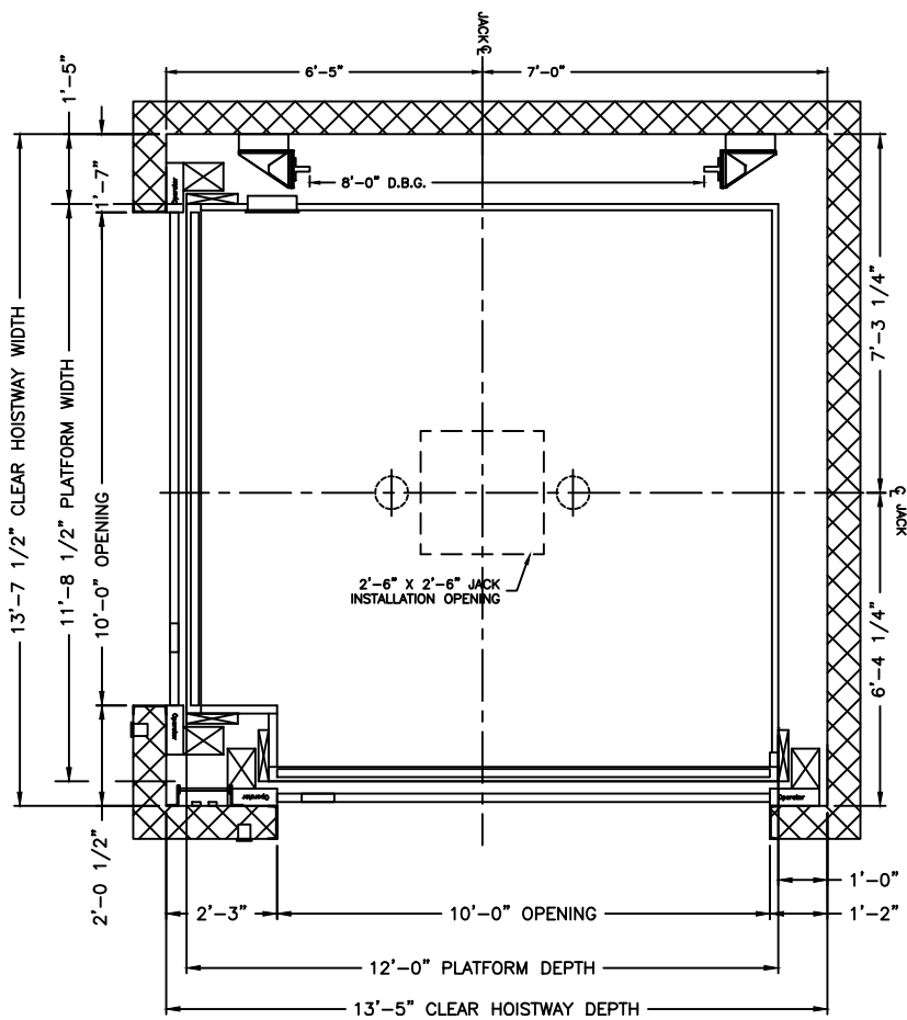
PLAN VIEW HOISTWAY
